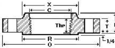
Threaded Flange
