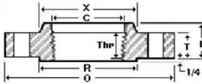
Threaded Flange
