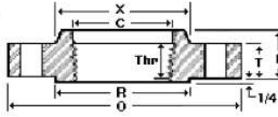
Threaded Flange
