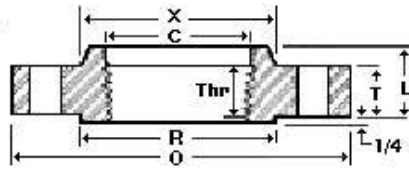
Threaded Flange
