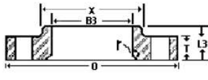
Lap Joint Flange
