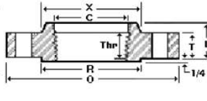
Threaded Flange
