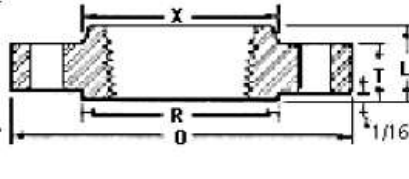
Threaded Flange
