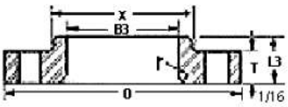
Lap Joint Flange
