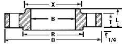
Slip On Flange
