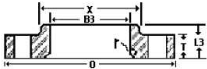
Lap Joint Flange
