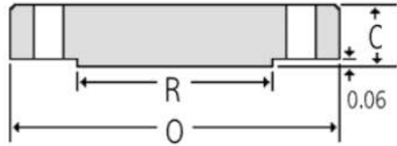
Blind Flange
