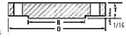
Blind Flange
