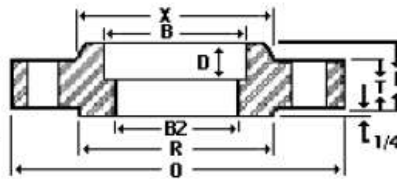
Socket Weld Flange
