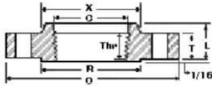
Threaded Flange
