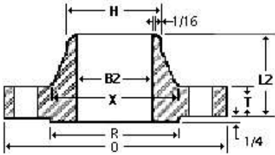
Weld Neck Flange
